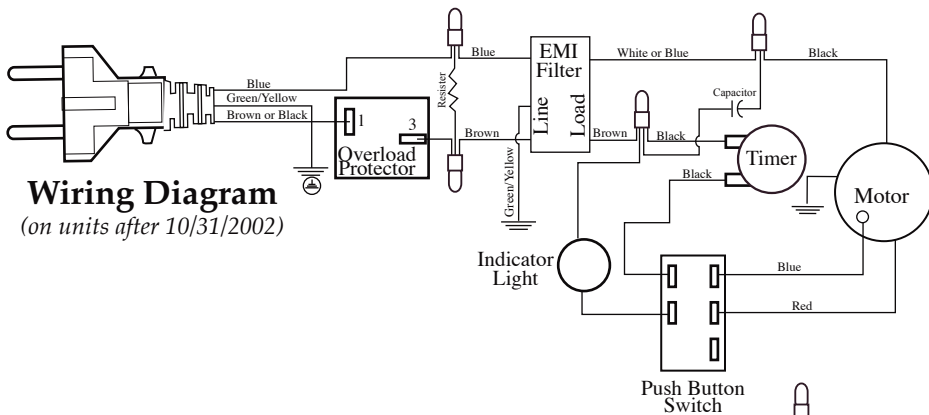
Wiring Diagram (on units after 1/12/2005)
